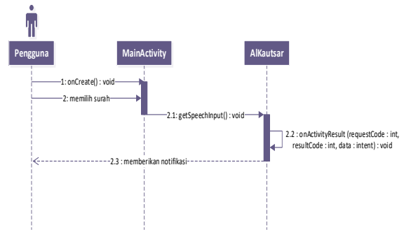
Gambar 3. Rancangan Sequence diagram
