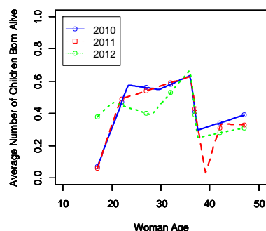
Figure 2 Spline Estimation Curves for Woman Fertility Data
