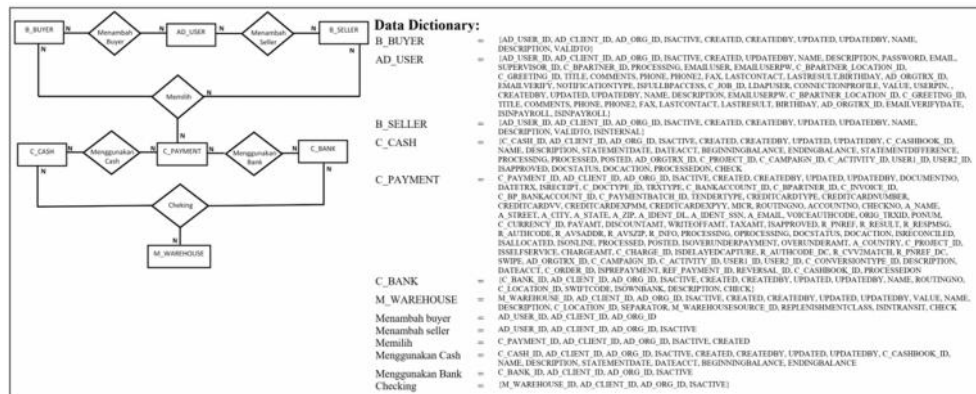
Figure 9. Data Dictionary in the E-R Diagram
