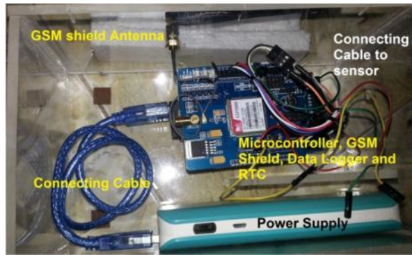
Figure 3. A prototype of data acquisition system.
