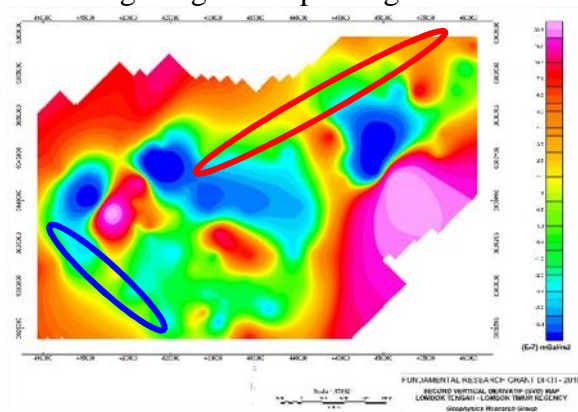
Figure 9. SVD map
