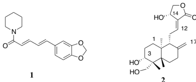
Figure 1. Structure of piperin (1) and andrographolide (2)
