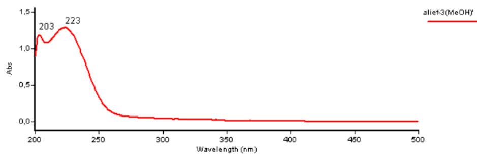
Figure 10. UV spectra of andrographolide
