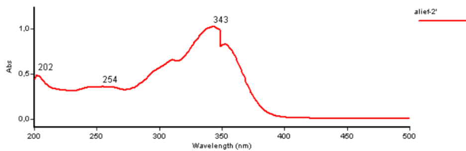
Figure 7. IR spectra of piperin
