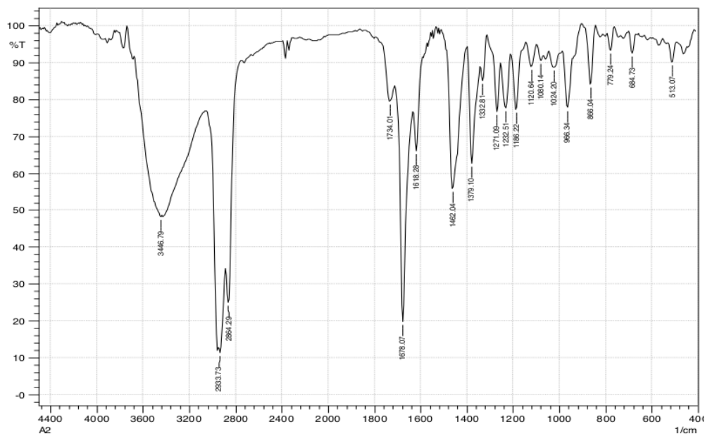
Figure 9. IR spectra of andrographolide
