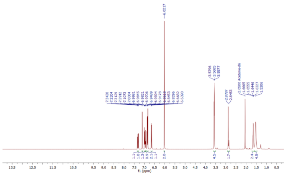
Figure 4. 1 H-NMR spectra of piperin
