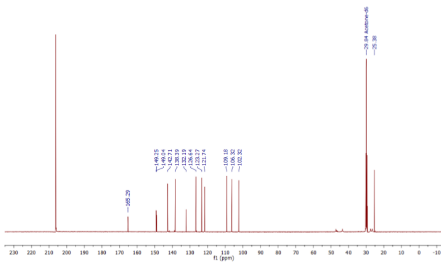
Figure 5. 13 C-NMR spectra of piperin
