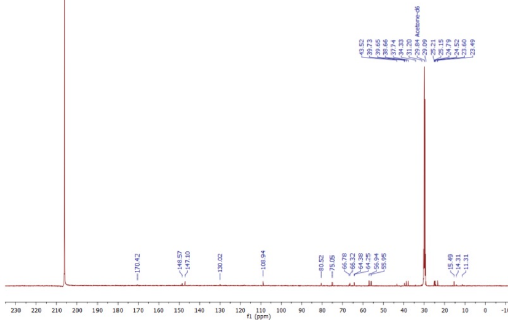
Figure 7. 13 C-NMR spectra of andrographolide
