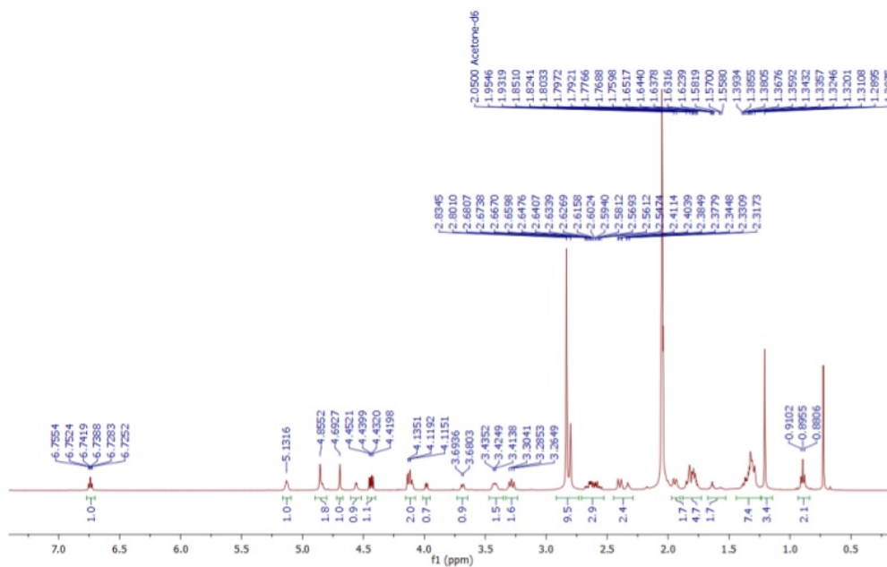
Figure 8. 1 H-NMR spectra of andrographolide
