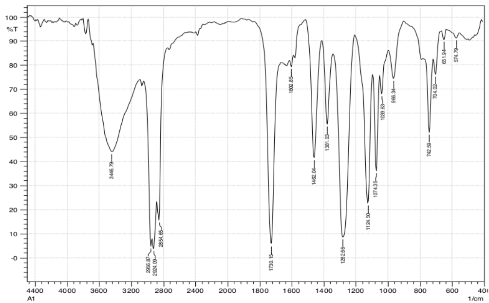
Figure 6. IR spectra of piperin
