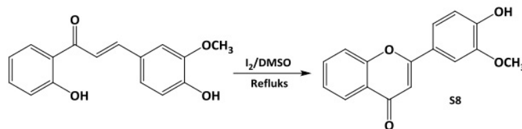
Figure 1. Pathway of synthesis of S8 compounds
