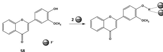
Figure 7. The S8 host-guest interaction model with F^- ions at a 1 : 2 stoichiometric ratio
