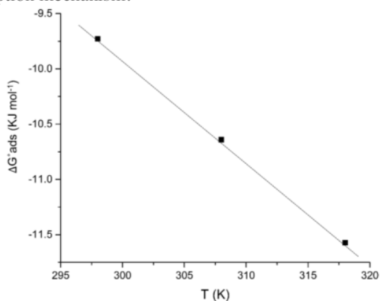
Figure 4. The relationship between \Delta G_{ads}^{\circ} and T for PN in 1 M HCl solution.
