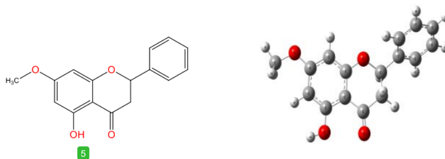
Figure 1. The structure of 5-hydroxy-7-methoxy-2-phenylchroman-4-one and the optimized structures of PN molecule determined using DFT method.
