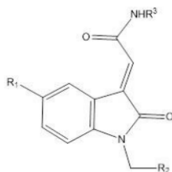
Figure 1. The parent compound of meisoindigo derivative
