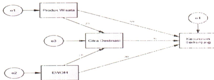
Gambar 4.1 Diagram Path
