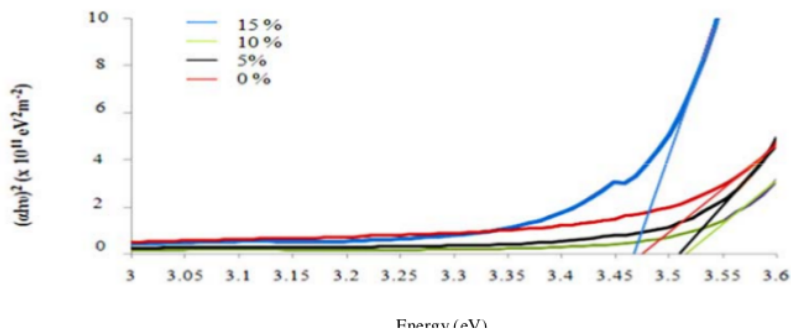
Figure 8. Energy gap SnO 2 and SnO 2 doped with 5%, 10%, and 15% Al on glass substrate
