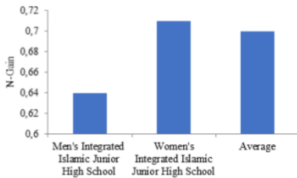
Fig. 2. Graphs of N-Gain Problem-Solving Capabilities.
