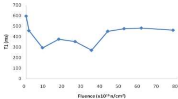
Gambar 3. Grafik waktu relaksasi spin-kisi (T1) metode pulsa 180^0\text{-}\tau\text{-}90^0 vs fluence neutron cuplikan polimer PVC.
