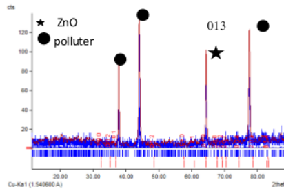
Figure 4. Thin layer ZnO, 0.1 M and temperature deposition at 550 °C of crystal diffraction intensity as a function of 2θ
