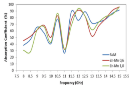
Fig. 4. The absorption coefficient (%A) of \text{BaFe}_{12-2x}\text{Zn}_x\text{Mn}_x\text{O}_{19} at 10-15 GHz.
