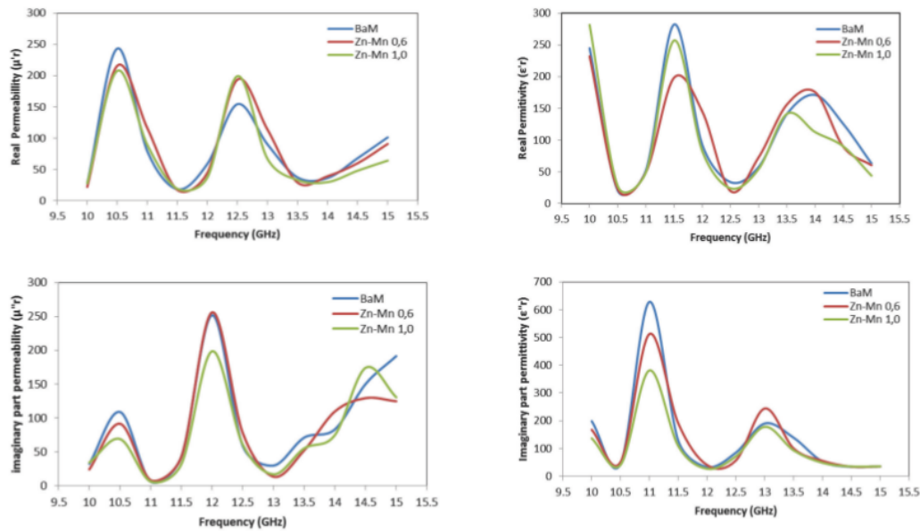
Fig. 3. The permeability and permittivity value of sample \text{BaFe}_{12-2x}\text{Zn}_x\text{Mn}_x\text{O}_{19} .
