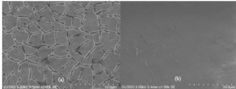
Fig. 1. Surface morphology of thin layer of tin oxide with doping (a) 0% Antimony and (b) 20% antimony.
