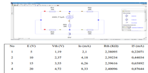
Figure 2. Example of Thevenin Circuit with LiveWire and Result Experiment
