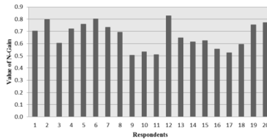
Fig. 1. Graph of the N-gain value of each respondent.
