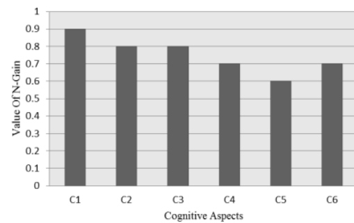
Fig. 2. Graph of the N-gain value of cognitive aspects.
