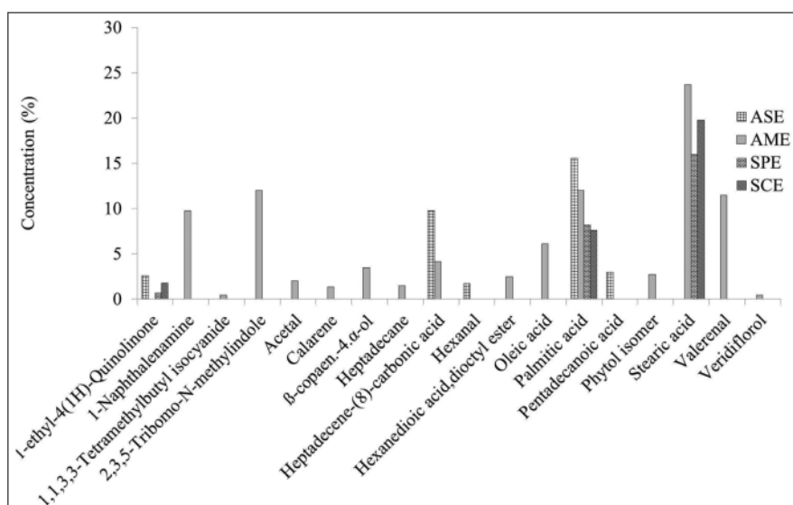
Figure 1. Chemical constituents of macroalgae crude ethanol extracts analyzed with GC-MS spectrometry.
