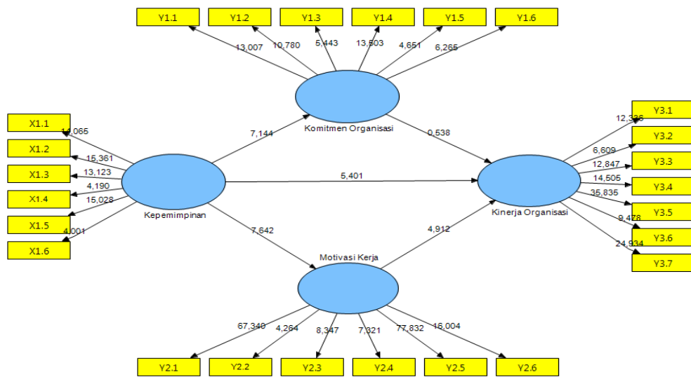
Gambar 4.2. Output Bootstrapping Model
