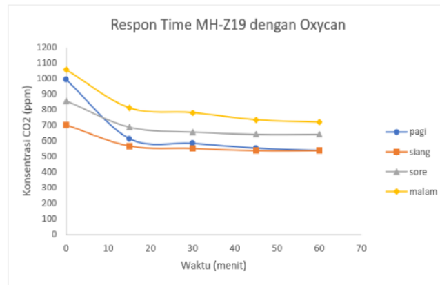
Gambar 4. Response time sensor terhadap pemberian Oksigen 95%.
