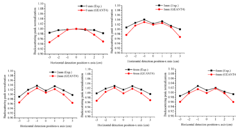
Figure 4. Backscattering peak normalization of A type design.
