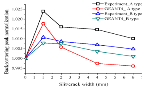
Figure 6. Backscattering peak normalization at x=0 detector position.
