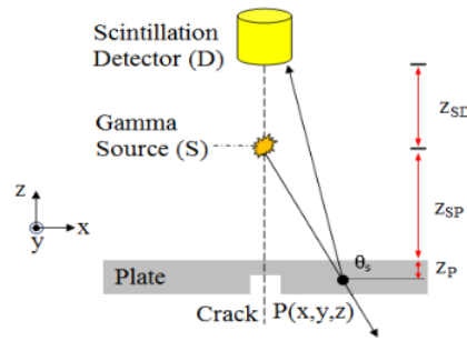
Figure 1. Gamma scattering from the plate model.
