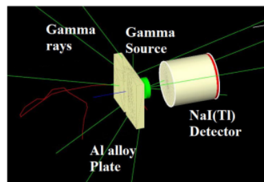
Figure 3. GEANT4 visualization of A type measurement.
