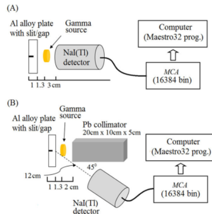
Figure 2. The schematic design of scattering measurement setup.
