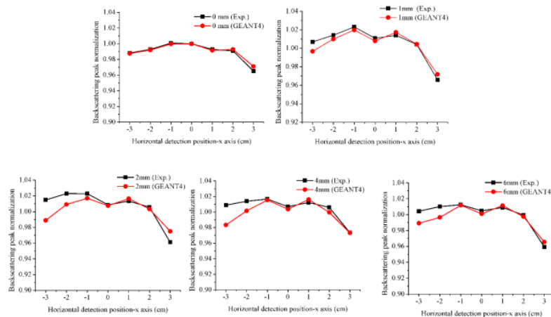
Figure 5. Backscattering peak normalization of B type design.
