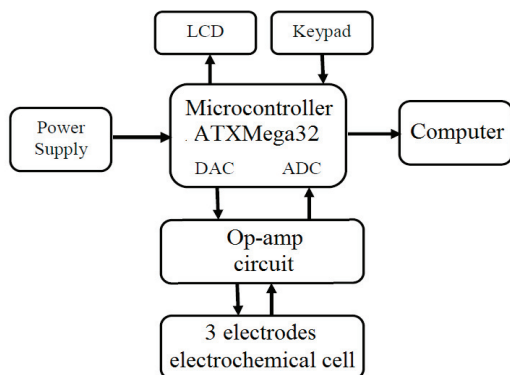
FIGURE 2. Diagram block of developed potentiostat system.
