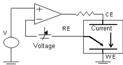
FIGURE 1. The scheme of potentiostat circuit.
