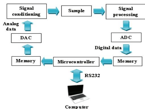
FIGURE 4. The developed potentiostat control system.
