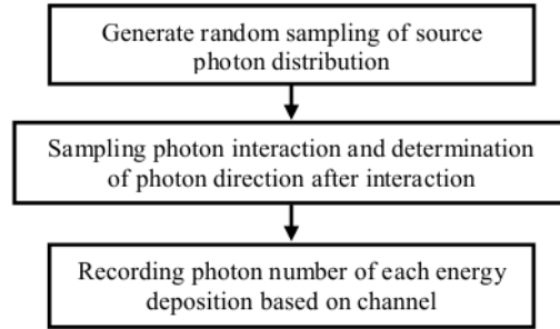
FIGURE 4. Three process Monte Carlo method.
