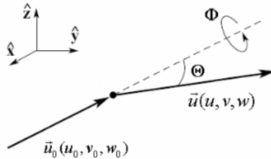
FIGURE 3. Photon deflection direction in single-scattering event.[5]
