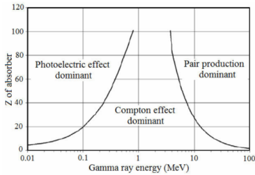
FIGURE 1. Three major types of gamma-ray interaction [1].
