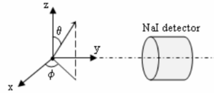
FIGURE 2. Coordinate system of photon generate
