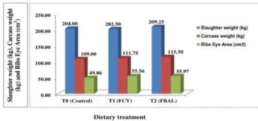
Figure 1. Graph of the relationship between the weight of the slaughter, the weight of the carcass and the eye rib area. The values are mean from four replication. FCY= Yeast Culture Fermentation; FBAL=Lactic Acid Bacteria Fermentation, T0=control, T1=first treatment, T2=second treatment, WHC=water holding capacity.
