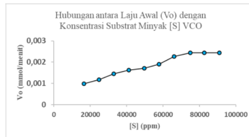
Gambar 2. Plot Michaelis-Menten
