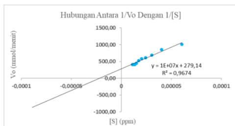
Gambar 3. Kurva Lineweaver-Burk
