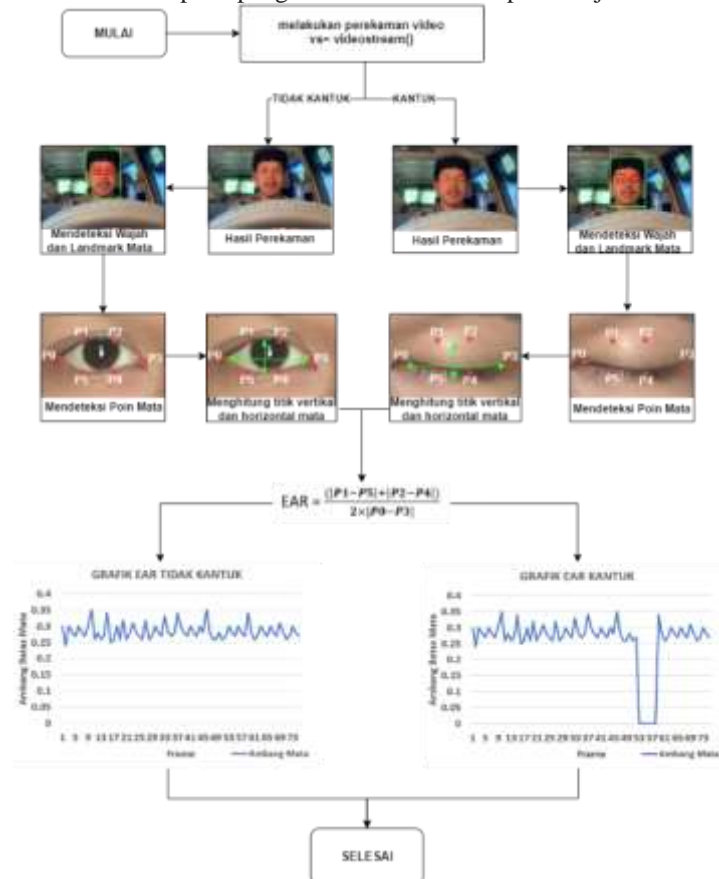
Gambar 8 Proses Eye Aspect Ratio
