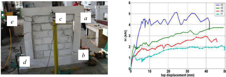
Fig. 1. Frame F1 under testing (left) and load-displacements of all test results (right)
