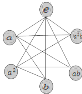
Figure 2.1 Coprime graph of dihedral group D_6
