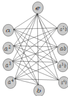
Figure 4.3 Coprime graph of dihedral group D_{10}
