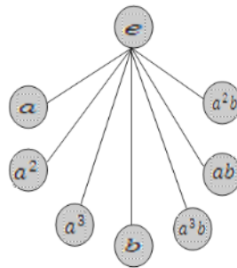
Figure 4.2 Coprime graph of dihedral group D_8
