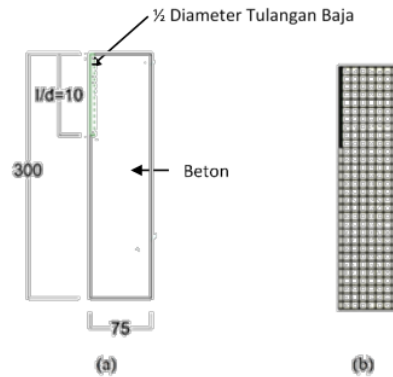
Gambar 6. Model axisymmetric (a) Geometri 2D (b) Meshing
