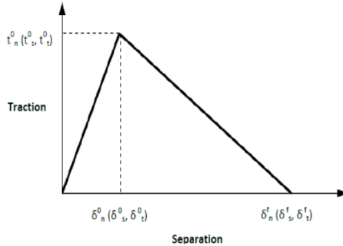
Gambar 2. Hukum traction separation (ABAQUS, 2018)
