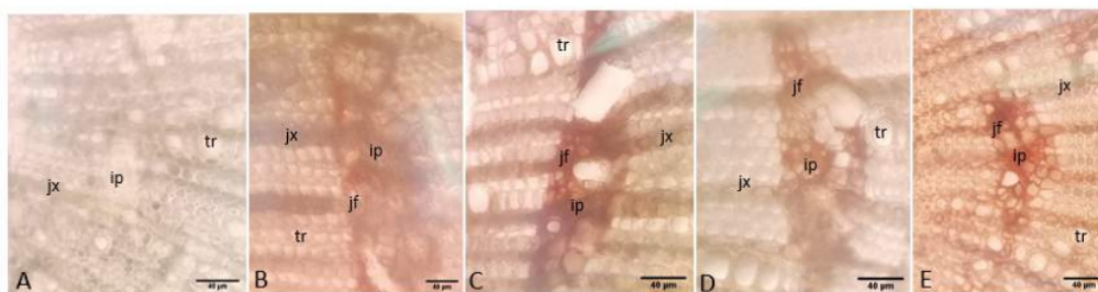
Fig. 3. Cross-section of the stem of a G. versteegii seedling inoculated with four different inducers aged 75 DAI: (a) healthy stems, (b) negative control, (c) liquid inducer, (d) gel inducer, (e) paste inducer, (f) ip = interxylary phloem, tr = trachea, jx = xylem pith radius, and jf = phloem pith fingers.
