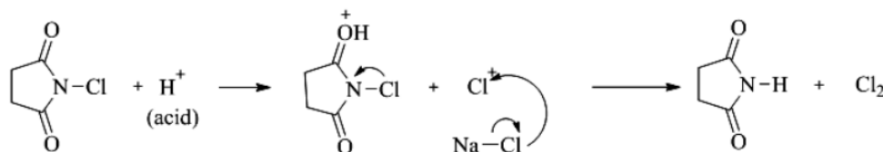
Scheme 2. Proposed reaction of chlorine formation from NCS.
