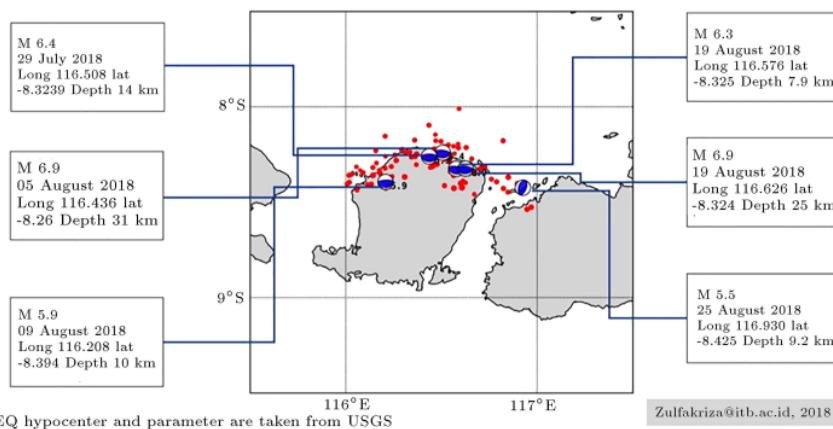
Figure 2. Distribution of Lombok earthquake occurrence [2].
