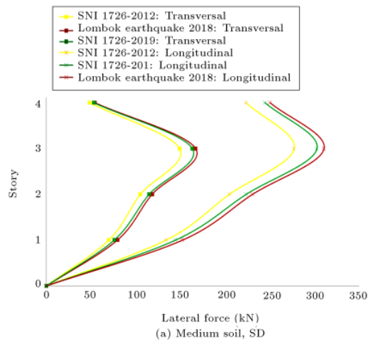
(a) Medium soil, SD
