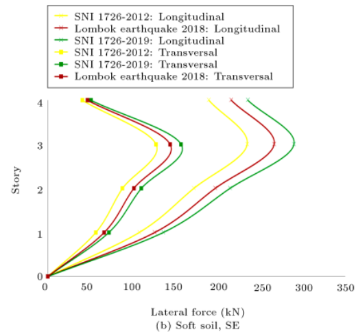
Figure 10. Lateral forces of the overviewed frame section.
