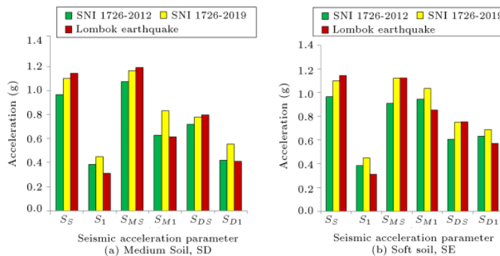
Figure 7. Spectral acceleration parameters.
