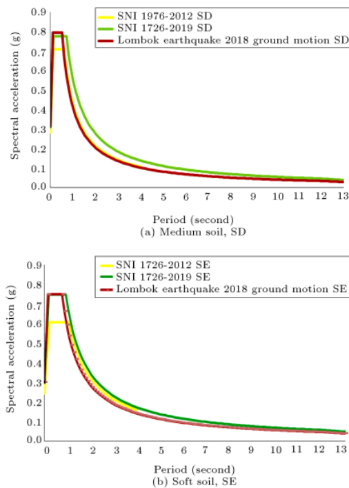
Figure 8. Response spectrum curve.
