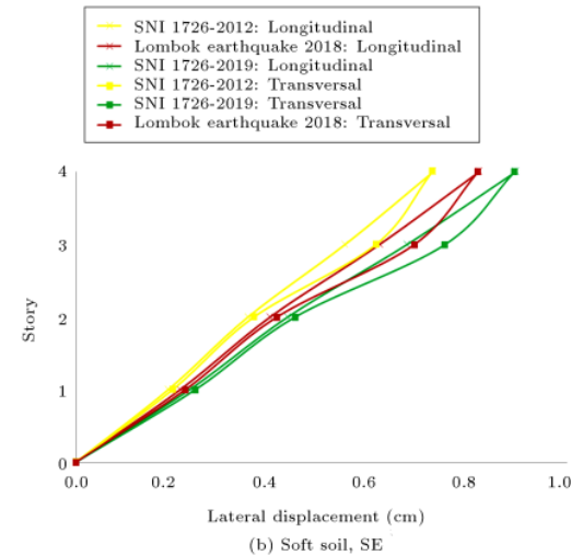
Figure 11. Lateral displacement of the overviewed frame section.
