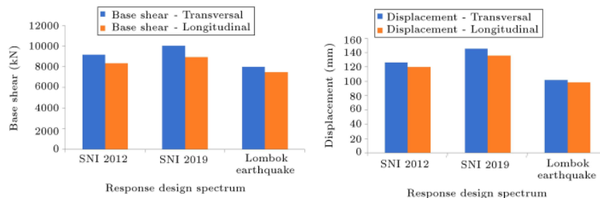
Figure 12. Performance point for base shear and displacement.
