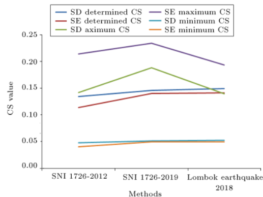
Figure 9. C_S value determined by the three approaches.
