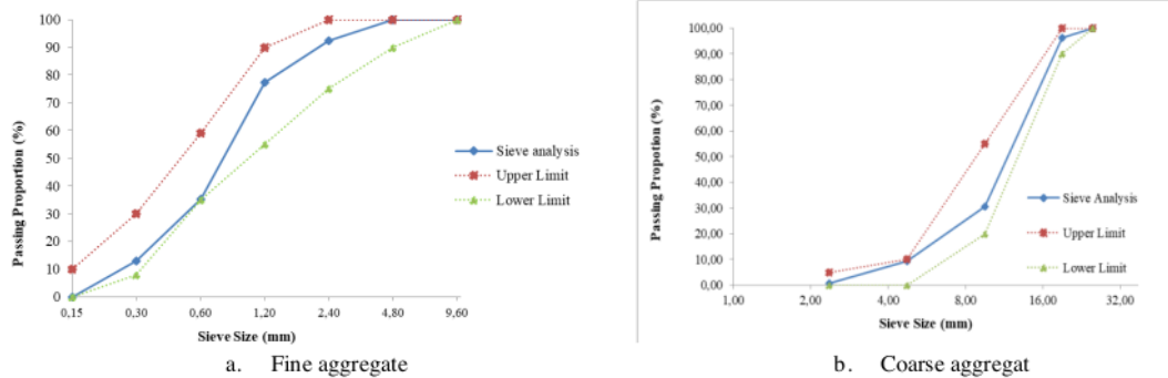
FIGURE 2. Sieve analysis
