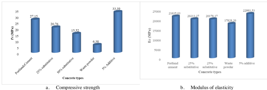
Figure 7. Mechanical properties
