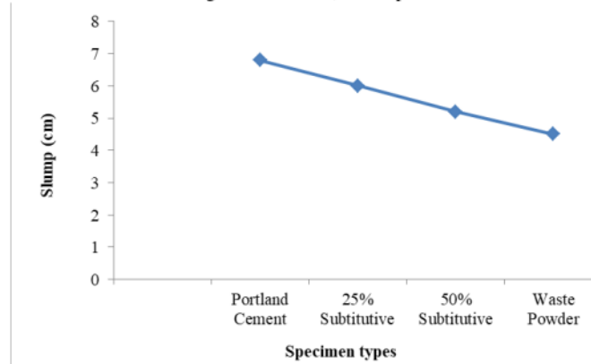
FIGURE 6. Fresh concrete slump
