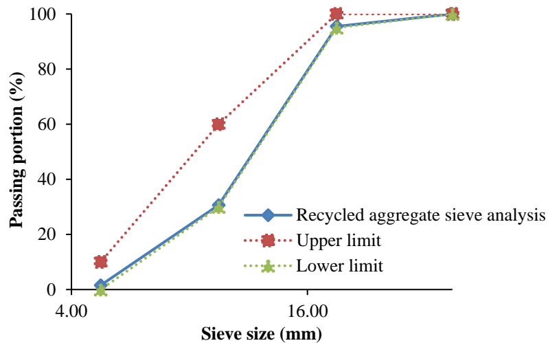
Figure 4. Sieve analysis of recycled coarse aggregate
