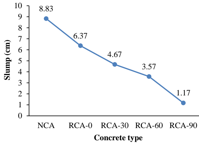
Figure 6. Concrete fresh properties
