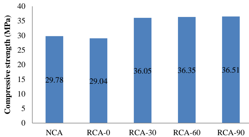
Figure 8. Concrete compressive strength
