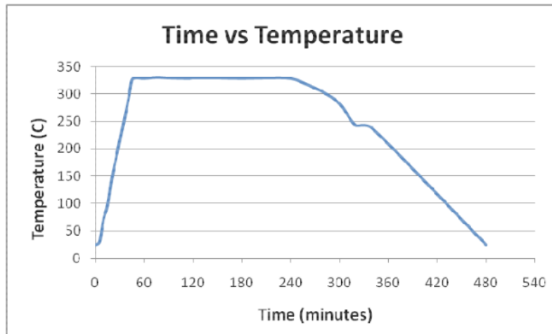
Figure 6. Time-Temperature of furnace up to 330°C
