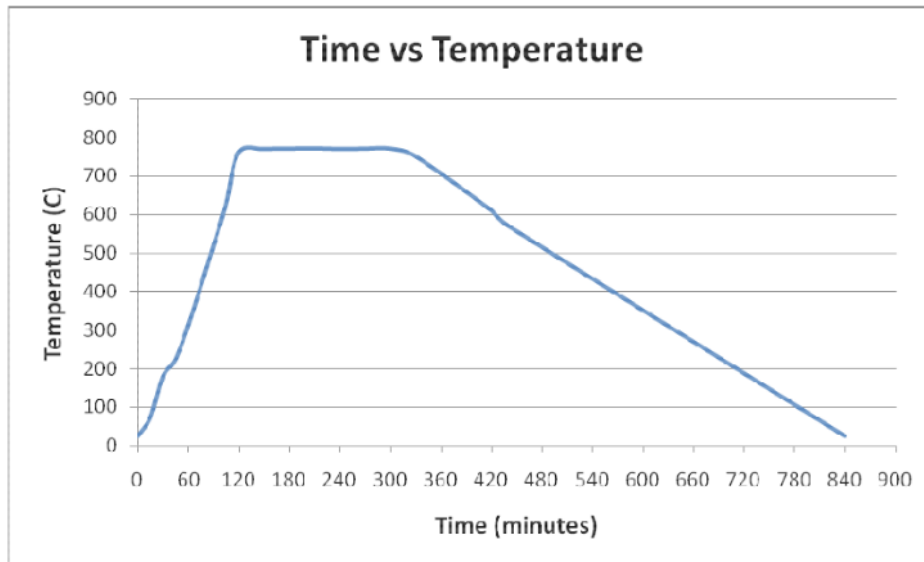
Figure 7. Time-Temperature of furnace up to 770°C
