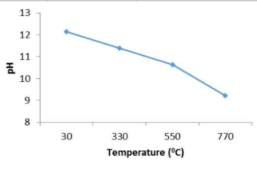
Gambar 4 Uji pH Beton Pasca bakar
