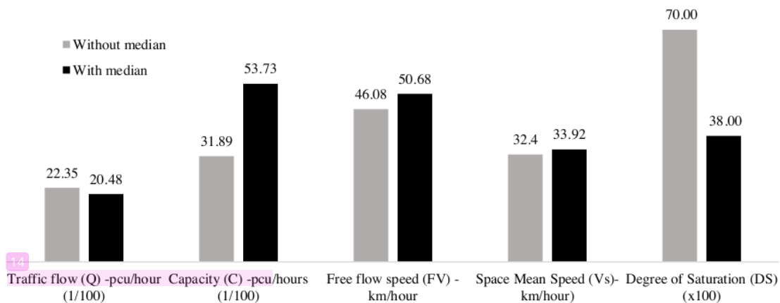
Figure 3: Section road performance parameters with and without median
