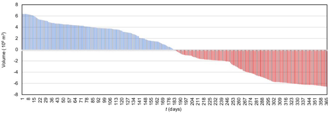
Fig. 7. Reliability of reservoir capacity during moderate El-Nino; source: own study
