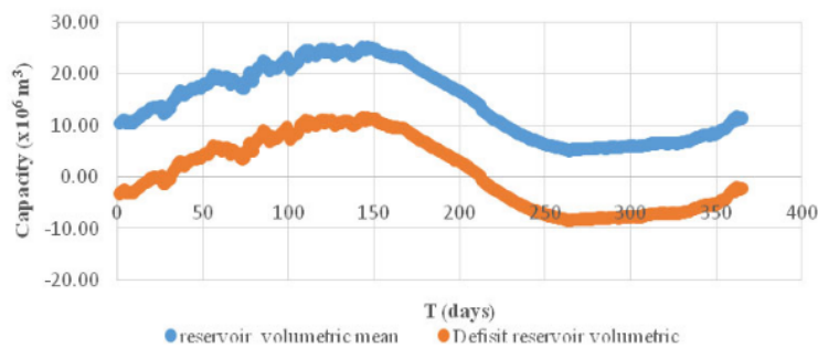
Figure 7 Average reservoir and deficit capacity of Mamak reservoirs at El Niño (see online version for colours)
