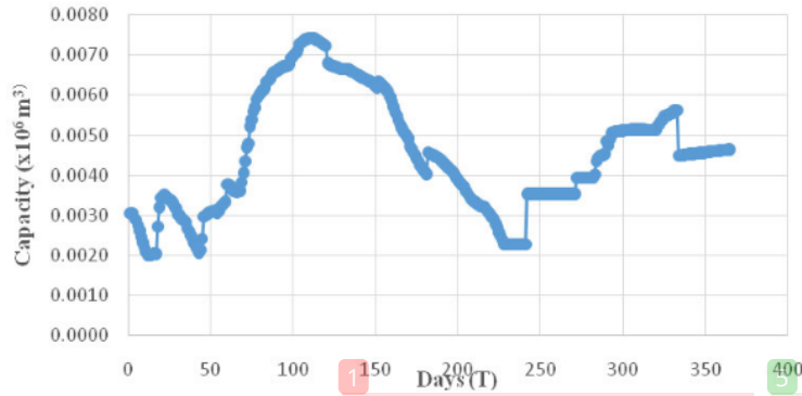
Figure 2 Average evaporation of the reservoir at the time of El Niño (see online version for colours)
