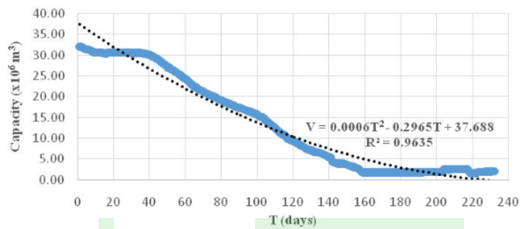
Figure 5 Decreasing line of reservoir capacity (see online version for colours)
