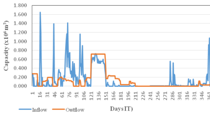
Figure 3 The average inflow and outflow of the reservoir at the time of El Niño (see online version for colours)
