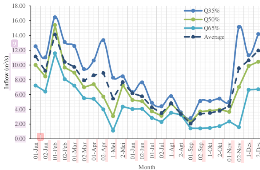
Figure 2 Scenarios of inflow discharge in the Batu Bulan Reservoir
