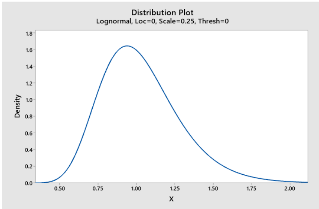
Figure 4. A PDF Plot of Lognormal Distribution
