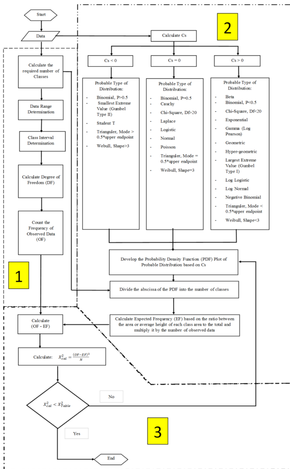
Figure 2. The Proposed Process Diagram
