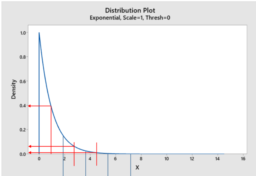
Figure 12. The height lines in the PDF data from Brewarrina
