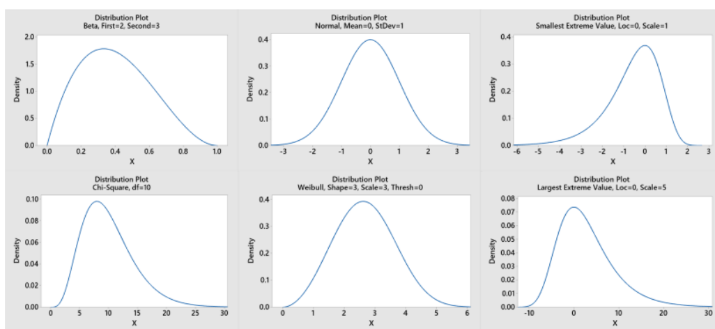
Figure 1. The Plots of Probability Density Function
