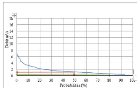
Gambar 1. Rerata Flow Duration Curve Pos Duga Air Kabupaten Bima
