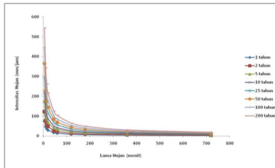
Gambar 4. Intensity-Duration-Frequency
