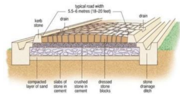
Gambar 1. Drainase Permukaan (Sumber : engineering.stackexchange.com )
