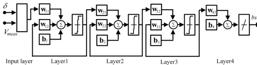
Figure 3. Architecture of SVC-LRN with 10-10-1-1 layers.
