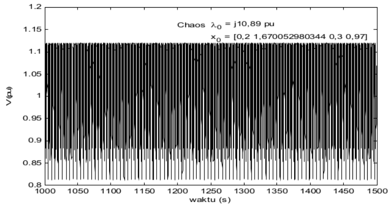
Figure 5. Chaos occurred in power systems
