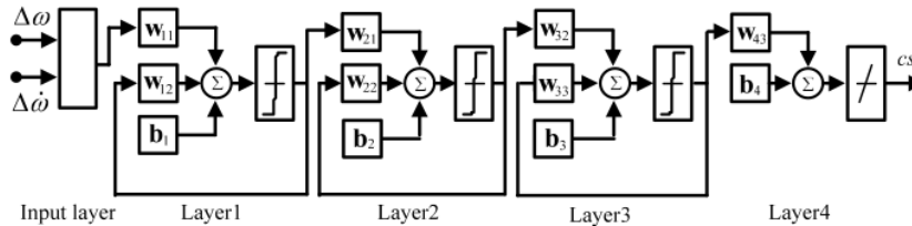
Figure 2. Architecture of PID-LRN with 10-10-1-1 layers.
