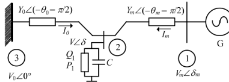
Figure 1. Three-bus power systems
