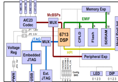
Gambar 1. Blok Diagram TMS320C6713
