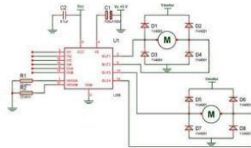
Gambar 6. Rangkaian Driver Motor DC
