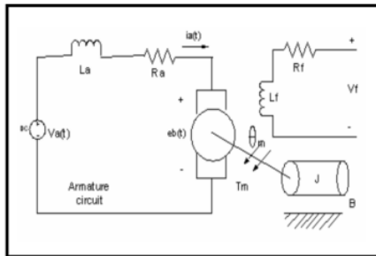
Gambar 3. Model rangkaian motor dc
