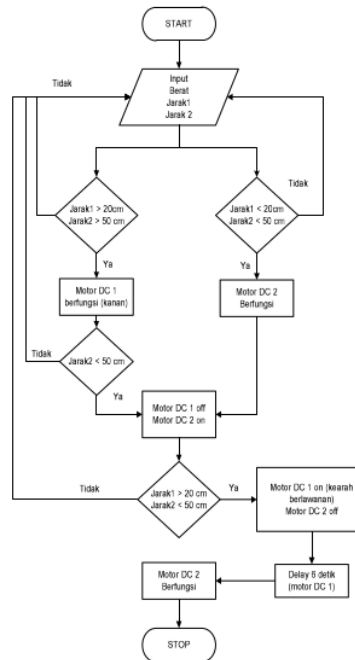
Gambar 8. Flowchart Program
