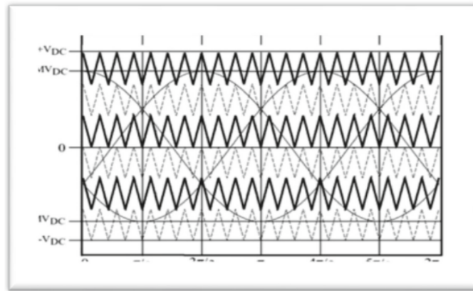
Fig. 4. CBPWM 7 level.
