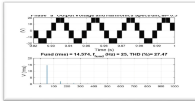
Fig. 10. Signal Output from Advance CBPWM.
