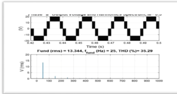
Fig. 11. Signal Output from CBPWM.
