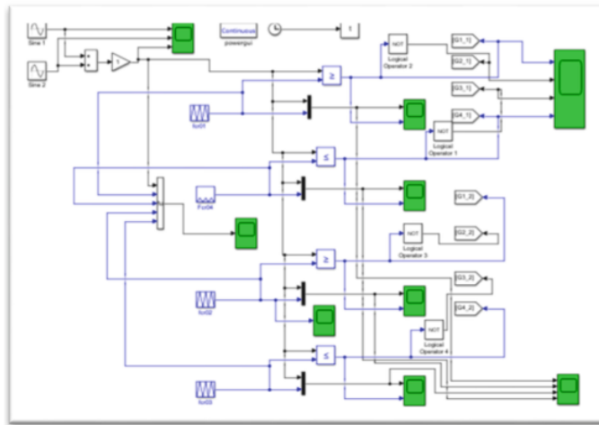
Fig. 8. Scheme Detail for ACBPWM.
