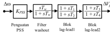
Gambar 6. Diagram blok power system stabilizer konvensional
