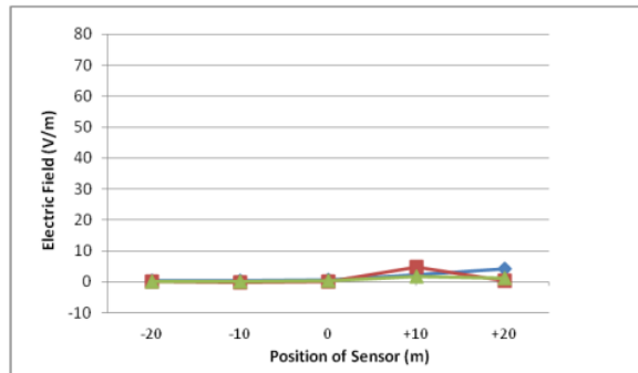
Fig. 3. Electric field measurements results on Residentials (blue= morning, red=midday, and green=night)
