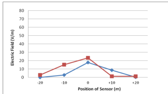
Fig. 4. Electric field measurements results on Gardens (blue= morning, red=midday)
