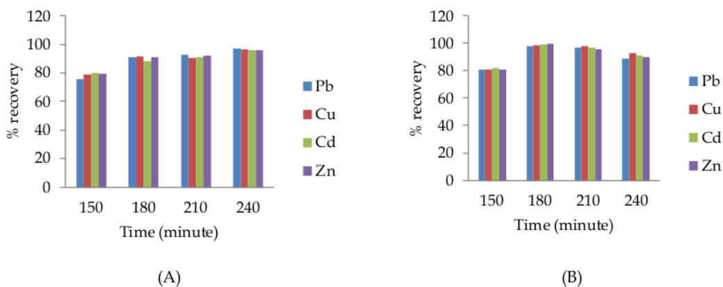
Figure 1. Effect of destruction time on % recovery of the destruction materials A: HNO 3 + H 2 SO 4 and B: HNO 3 + H 2 SO 4 + HClO 4
