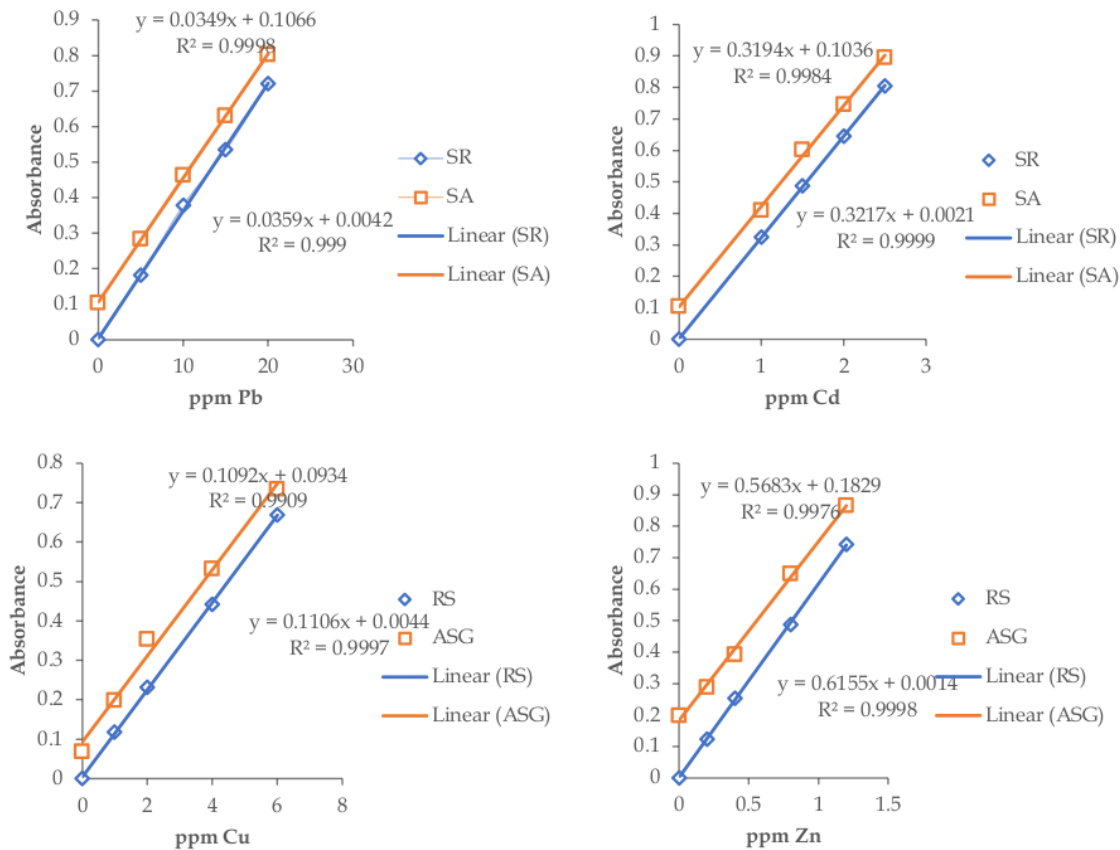
Figure 2. Standard Regression (SR) and Standard Addition (SA)
