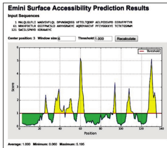
Figure 3. The results of the analysis of the BSP-1 Epitope prediction based on the IEDB. Predicted Emini surface accessibility of the proposed epitope, with a minimum propensity score of 0.060 and a maximum score of 5.195. Sequence positions and surface probabilities are directed by the X- and Y- axes, respectively. The areas above the threshold are antigenic, shown in yellow.
