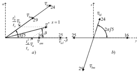
Fig. 2. Principle of calculation of times of application of the active space vectors in the \alpha - \beta (a) and x - y (b) planes.
