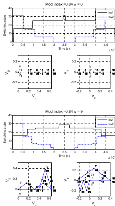
Fig. 8: Inverter switching trajectories in the \alpha - \beta and x - y planes for M = 0.84 and reference angular positions of 0^\circ and 9^\circ in the \alpha - \beta plane.
