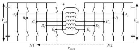
Fig. 3. Five-phase machine with dual two-level inverter supply.
