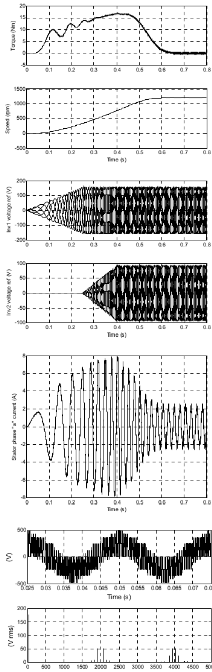
Fig. 7: Motor acceleration under V/f control (ref. 40Hz, M = 0.84 ): speed, torque, inverter voltage references, stator current and steady-state phase voltage waveform with spectrum.
