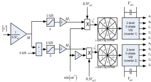
Fig. 5. Unequal reference sharing scheme.
